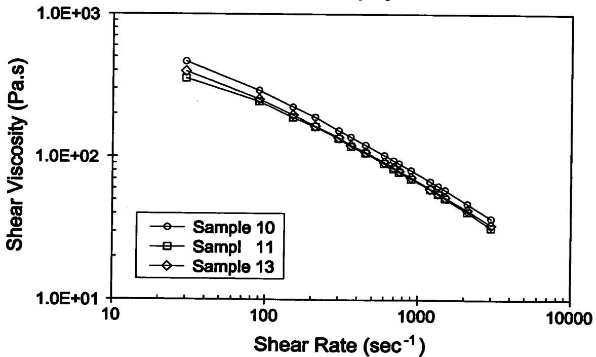
Fig. 12 Shear Viscosity of Plasticized Propylene Random Copolymers
